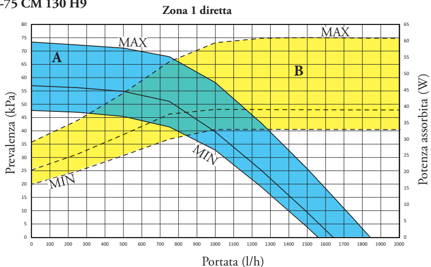
UPM3 K AUTO 15-75 CM 130 H9
